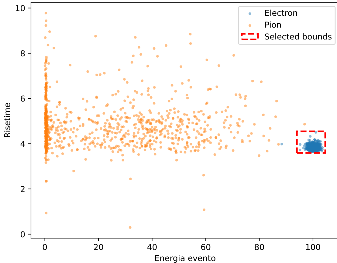
Scatter plot e/pi (all) 100.0GeV
