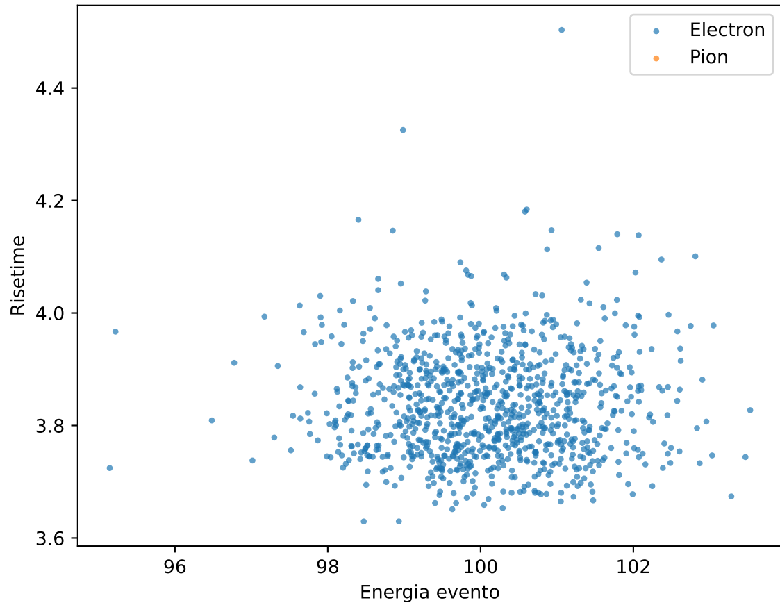
Scatter plot e/pi (cutted) 100.0GeV
